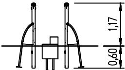
5 54 000 0 eibe fit Aktiv-Station stepped path 1:100
