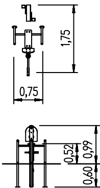
5 54 004 0 eibe fit Aktiv-Station sit-up bike 1:100
